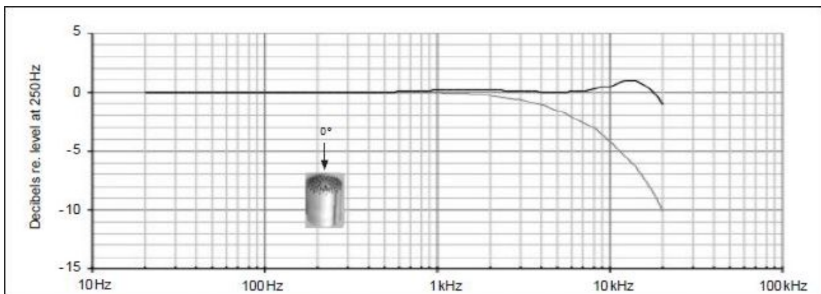
Typical frequency response. Upper curve shows free-field response for 0°, lower curve shows pressure
